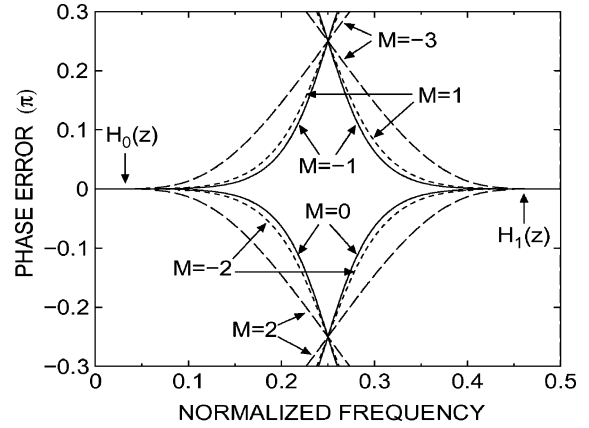
Fig. 4. Phase errors of H_0(z) and H_1(z) in Example 1.
